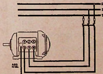
Fig. 2. Motor in sterschakeling.
