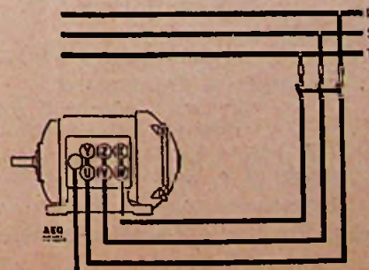
Fig. 3. Motor in driehoekschakeling.
